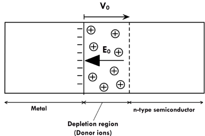
Figure 7: Schematic showing the metal, n-type semiconductor in contact, and the Schottky junction between them. There is a depletion layer in the n-type semiconductor due to transfer of electrons to the metal. This leads to the formation of a contact potential.
