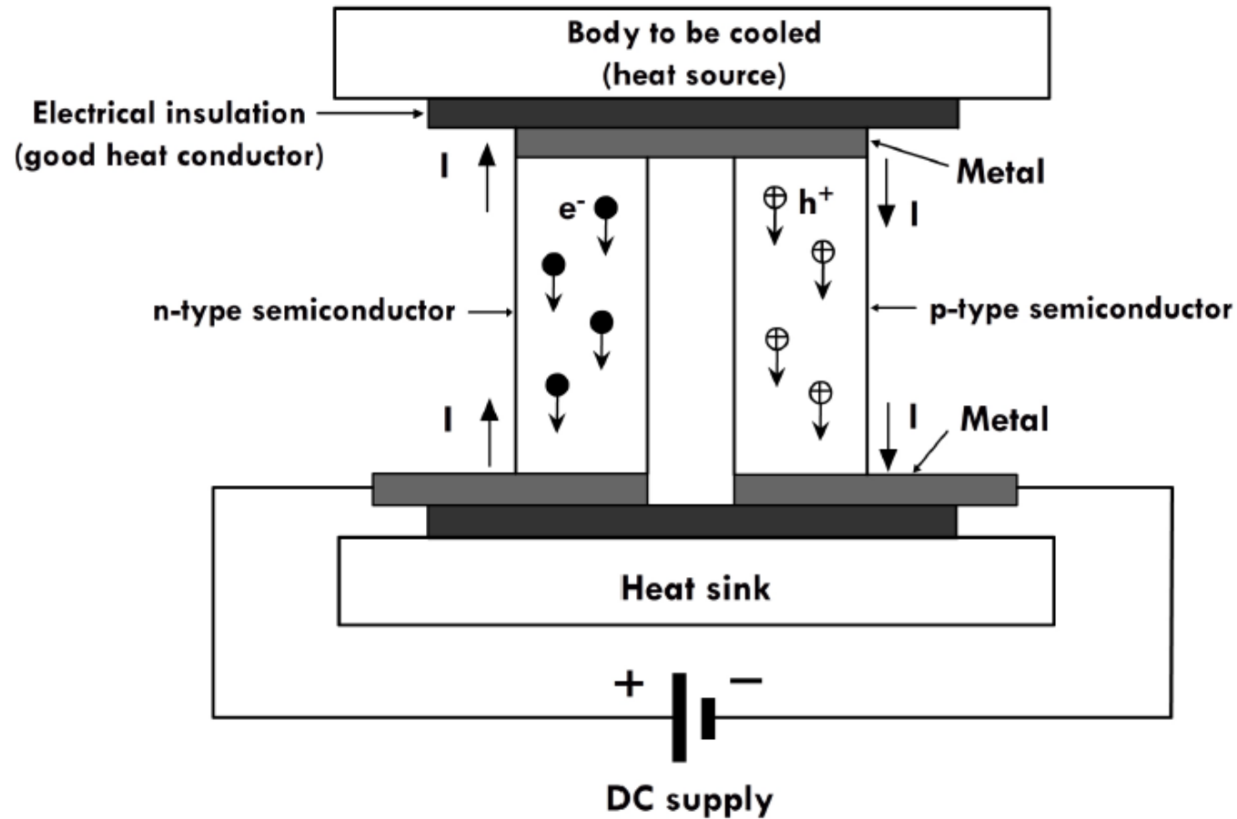
Figure 15: Schematic of the Peltier cooler using both p- and n- type semi-conductors. One end of the cooler is connected to the body from which heat is absorbed (cooled) and the other end is connected to a heat sink, where it is released
