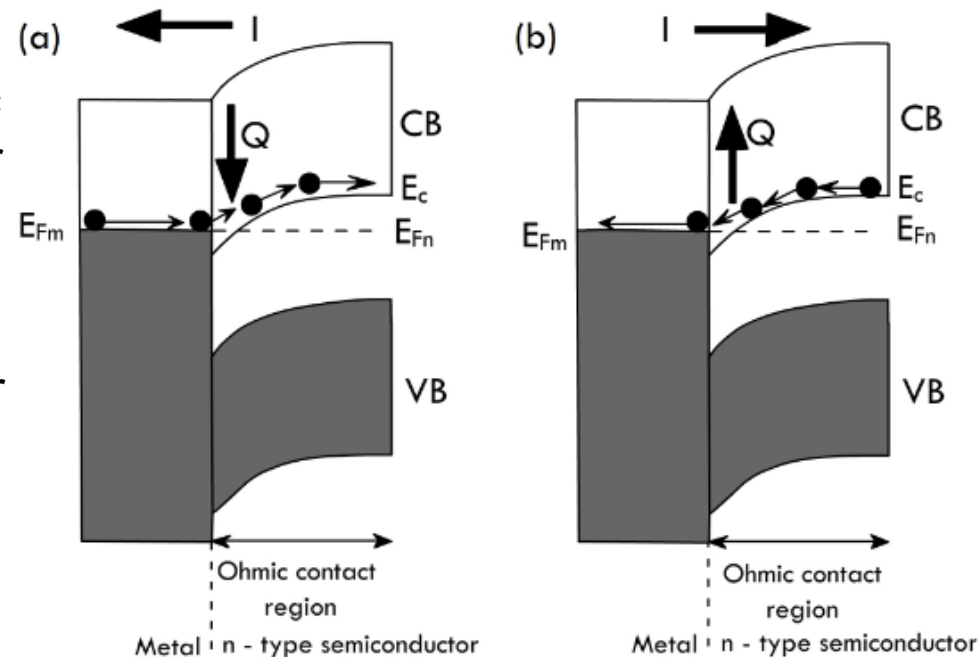
Figure 14: Current flow through an Ohmic junction can lead to heat (a) absorption or (b) release. This depends on the external bias, that determines the direction of heat flow. When electrons move from metal to higher energy levels in the semiconductor heat is absorbed from metal by electrons and the reverse happens when electrons flow from semiconductor to metal heat is released to metal by electrons
